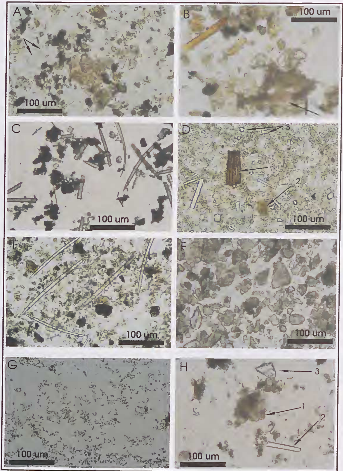
Figure 6. Annotated photomicrographs of standard particles in the fine-grained fraction of wetland sediments. Scale bar on all photomicrographs is 100 µm. Photomicrographs of the sand fraction is with reflected light through a stereoscopic microscope using a black background to the slide. All photomicrographs of the fine-grained fractions are using plane polarised transmitted light, except for (G), in which the light is partly cross-polarised. A. Organic matter (honey brown) in peat from Karrinyup Road Swamp, with scattered diatom debris (arrowed). B. Organic matter (brown and light honey brown) in peat from Karrinyup Road Swamp, with vestiges of cellular structure (arrowed) in the plant matter. C. Organic matter (dark particles) and sponge spicules and their fragments in peat from the shore of Lake Joondalup. D. Cellular plant material (arrow 1), homogenous plant material (arrow 2), quartz silt (arrow 3), and fragments of sponge spicules in a matrix of diatom silt; sample is the interstitial material from a diatomaceous peaty quartz sand. E. Sponge spicules in a diatom silt; sample of diatomite from wetland basin within Bassendean Dunes area east of Yanchep. F. Interstitial material from a kaolinitic muddy sand; the dominant mineral is kaolinite, with scattered quartz silt. G. Fine-grained calcite particles from a calcilutite, Lake Coogee. H. Carbonate intraclast (arrow 1), broken sponge spicule (arrow 2), and quartz silt (arrow 3) from a carbonate intraclastic sediment from Lake Coogee.
